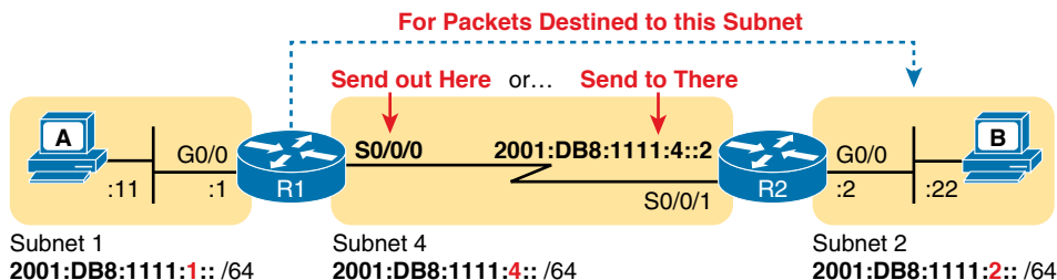
Figure 25-2 Logic Behind IPv6 Static Route Commands (IPv6 Route)
