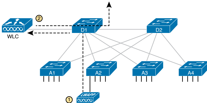
Figure K-20 Campus LAN, Multiple Lightweight APs, with Roaming
