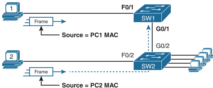
Figure 6-1 Source MAC Addresses in Frames as They Enter a Switch
