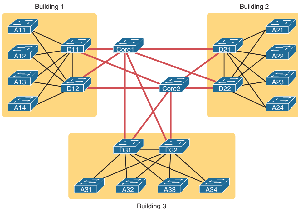
Figure 13-5 Three-Tier Building Design (Core Design), Three Buildings
