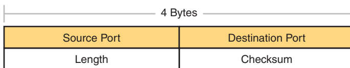
Figure 1-10 UDP Header
