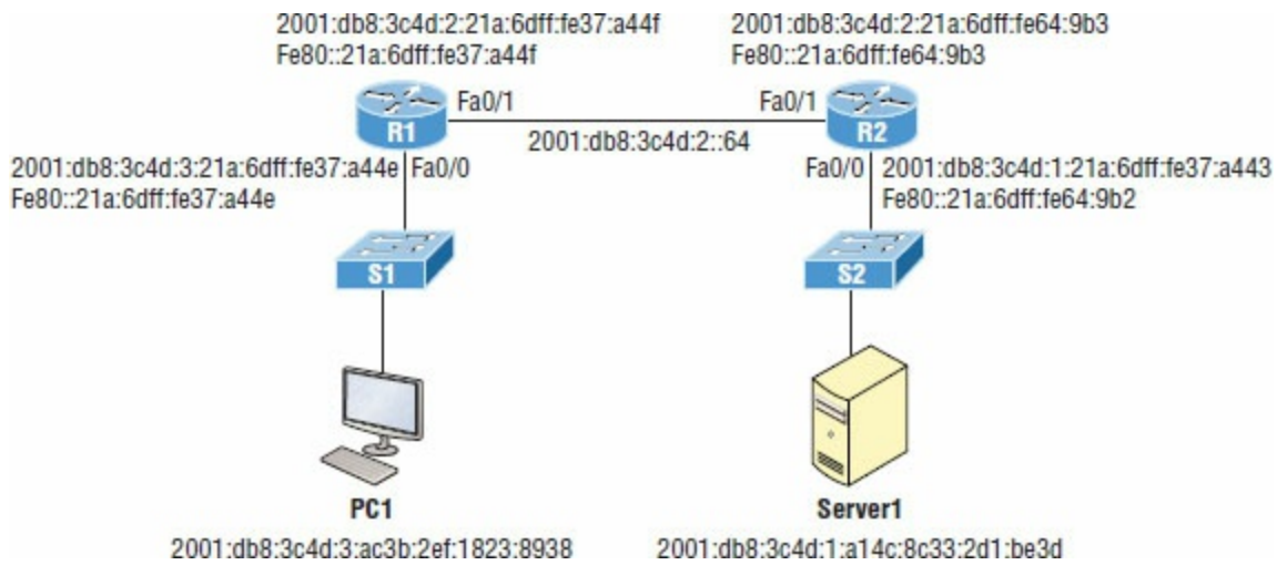
Figure 20.4 IPv6 troubleshooting scenario
