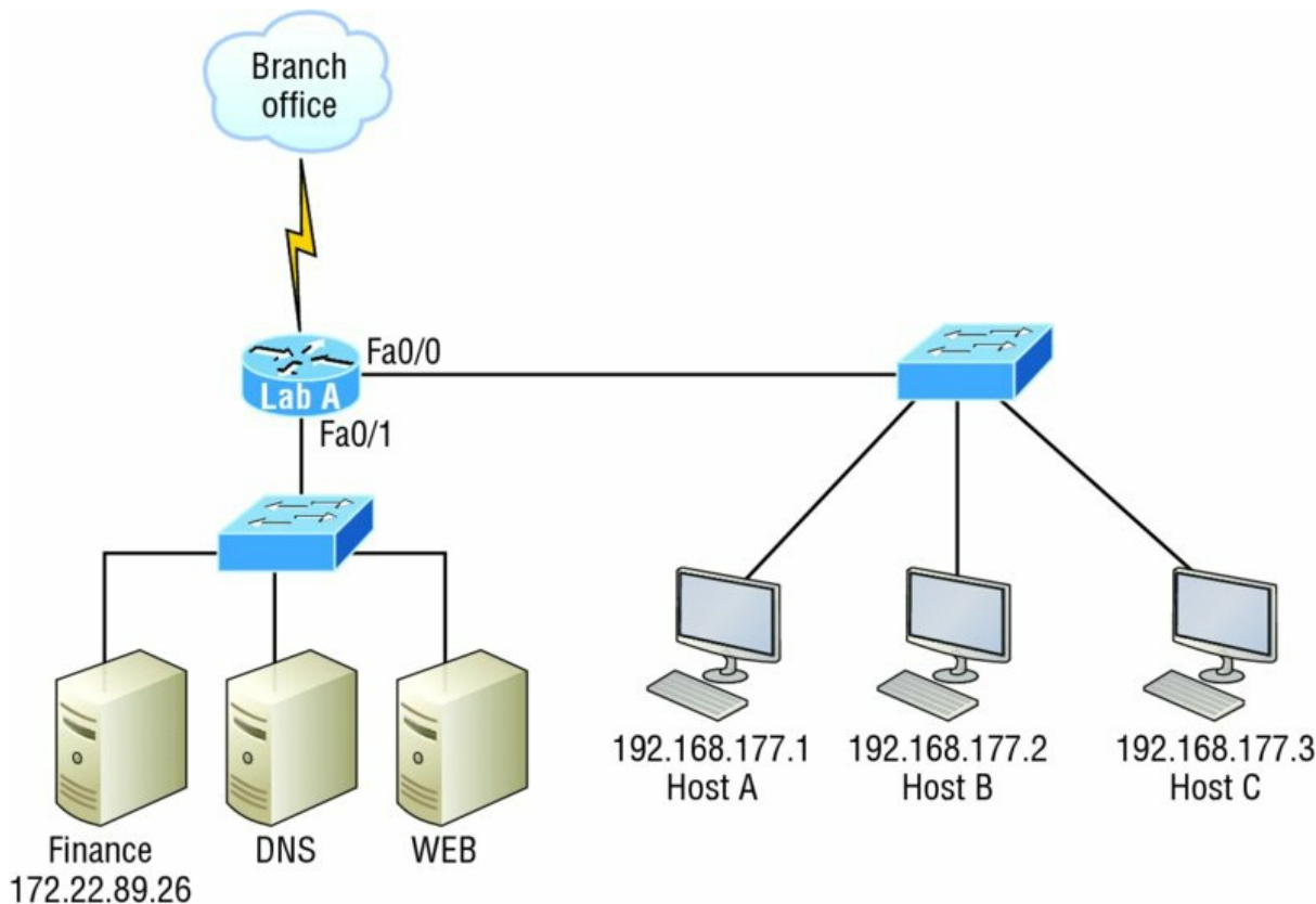
FIGURE 12.6 Extended ACL example 3
