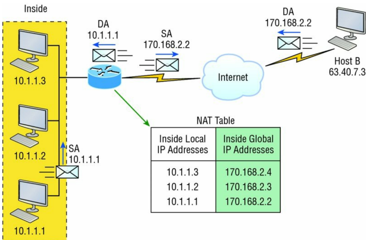
FIGURE 13.2 Basic NAT translation
