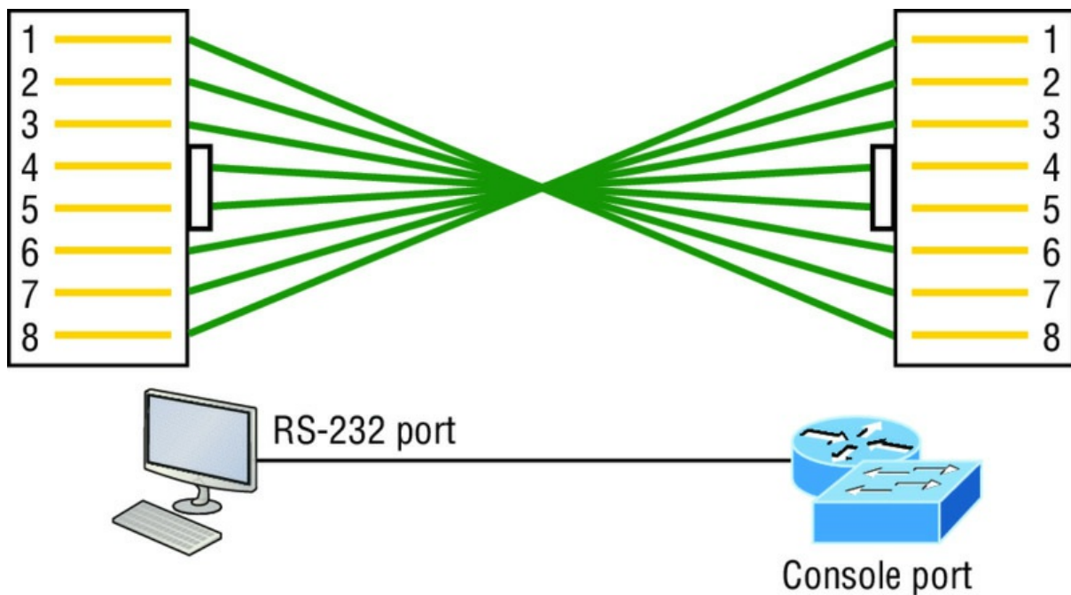
FIGURE 2.14 Rolled Ethernet cable
