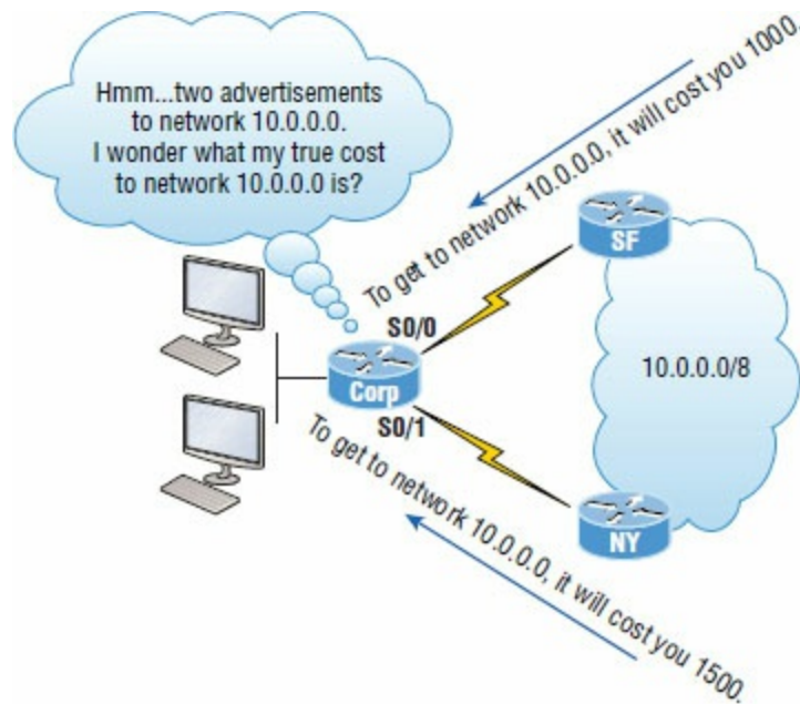
FIGURE 17.2 Advertised distance
