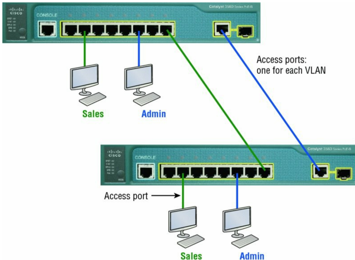
FIGURE 11.5 Access ports
