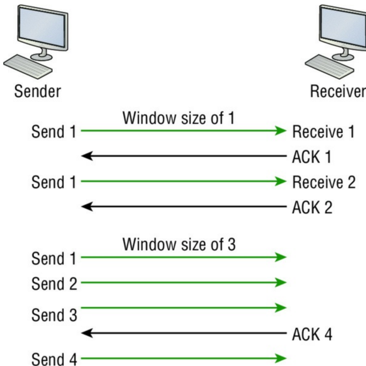
FIGURE 1.12 Windowing
