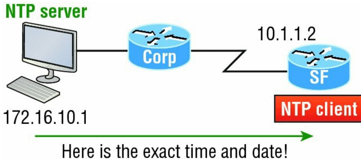
FIGURE 7.5 Synchronizing time information
