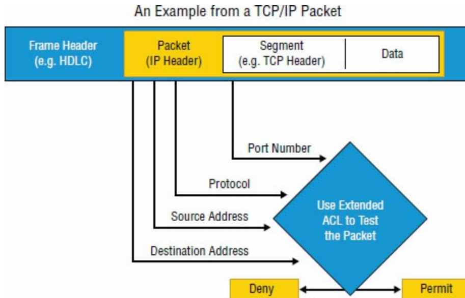
Figure 20.3 Extended ACLs
