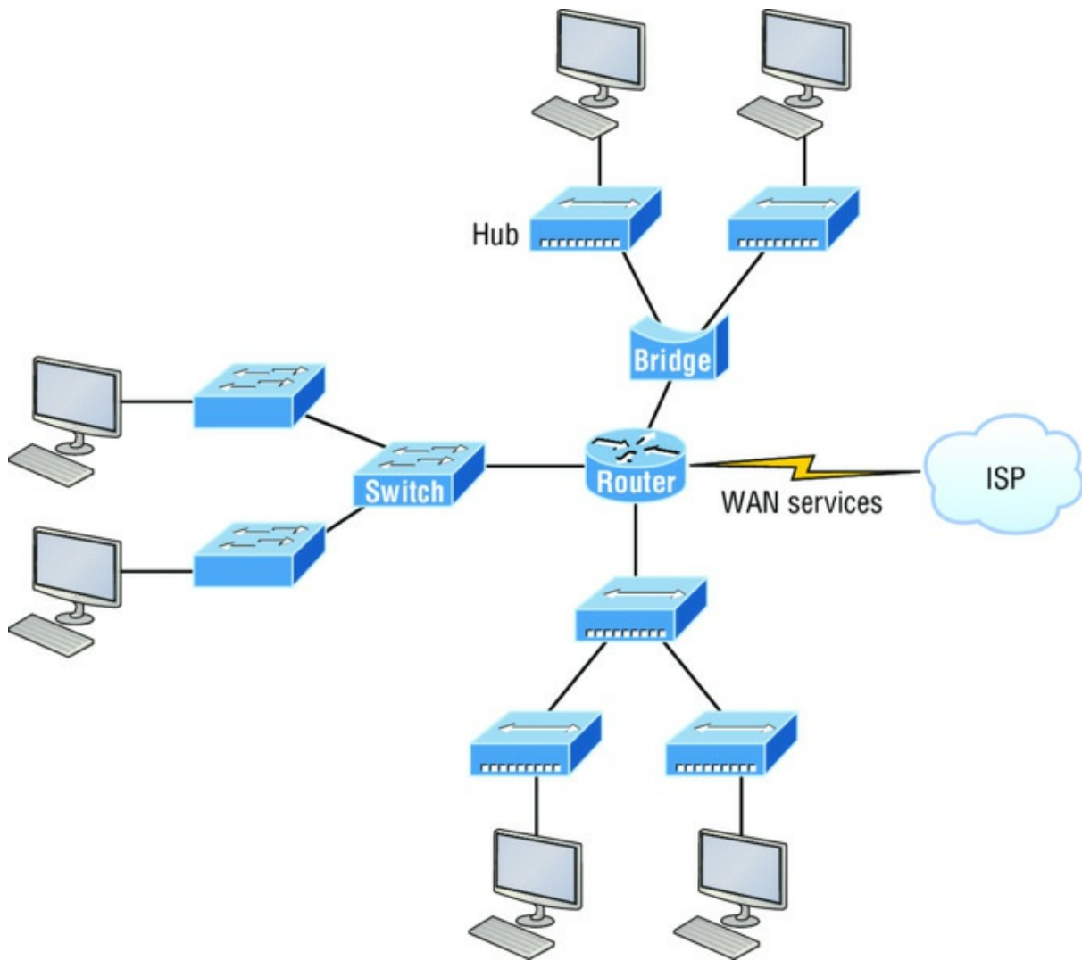
FIGURE 1.4 Internetworking devices
