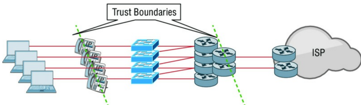
FIGURE 22.13 Trust boundaries
