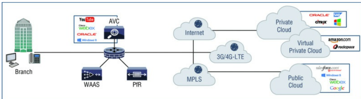
FIGURE 21.7 Intelligent WAN
