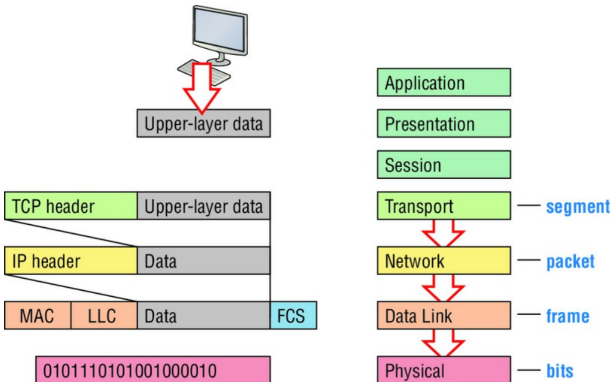
FIGURE 2.21 Data encapsulation
