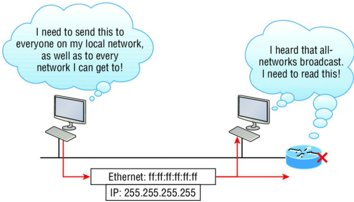
FIGURE 3.22 Layer 3 broadcasts
