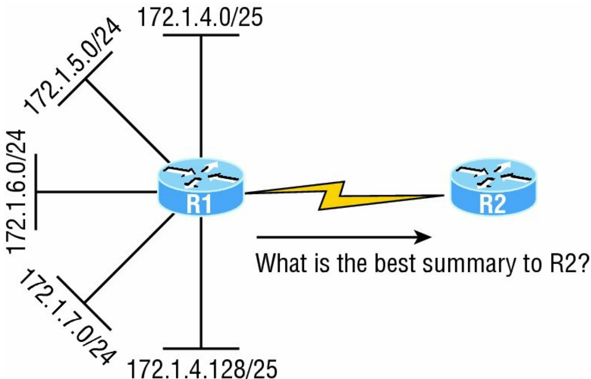
FIGURE 5.14 Summarization example 5
