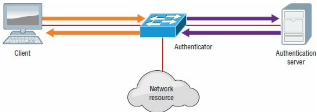
Figure 16.3 Identity-based networking
