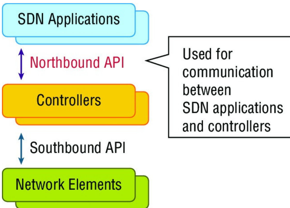
FIGURE 22.7 Northbound interfaces
