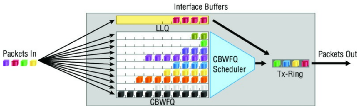
FIGURE 22.16 Queuing mechanisms
