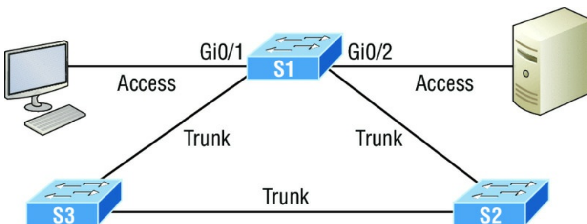
FIGURE 15.19 PortFast
