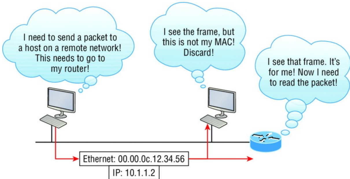
FIGURE 3.23 Unicast address
