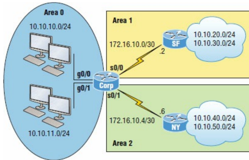
Figure 19.8 Our internetwork
