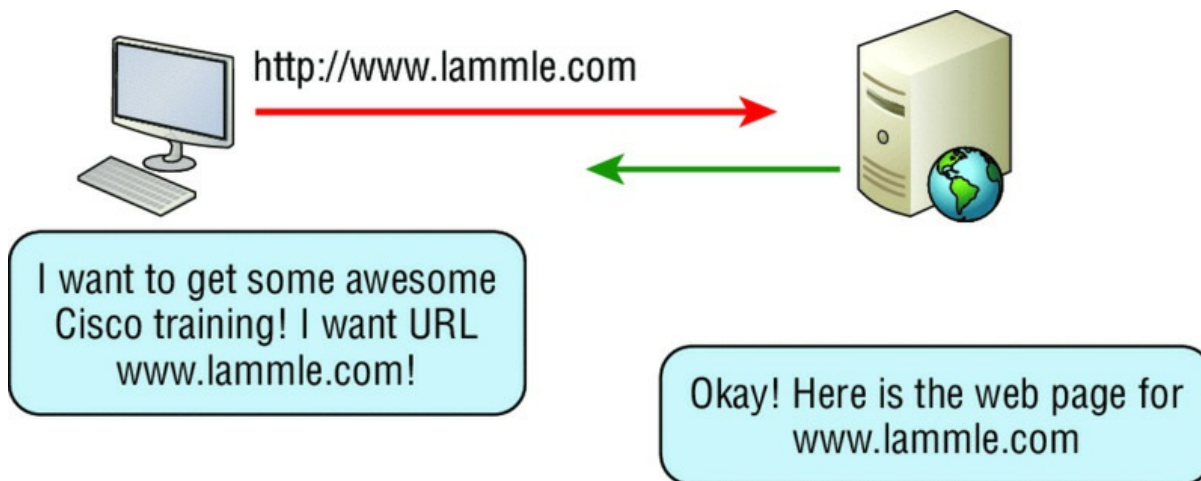
FIGURE 3.8 HTTP
