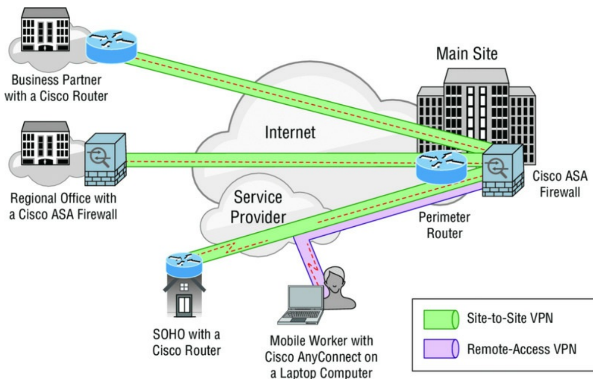
FIGURE 21.21 Enterprise-managed VPNs
