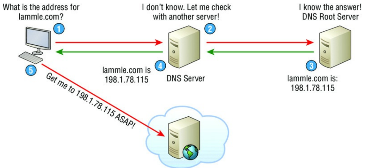
FIGURE 3.10 DNS
