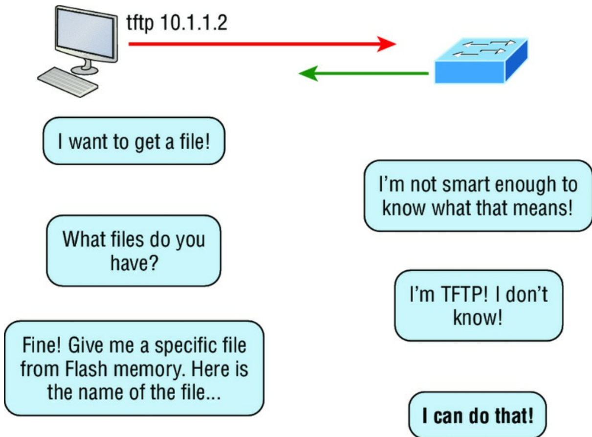
FIGURE 3.6 TFTP
