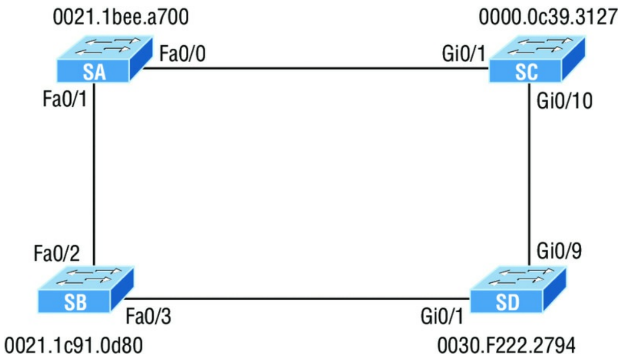
FIGURE 15.11 RSTP example 1
